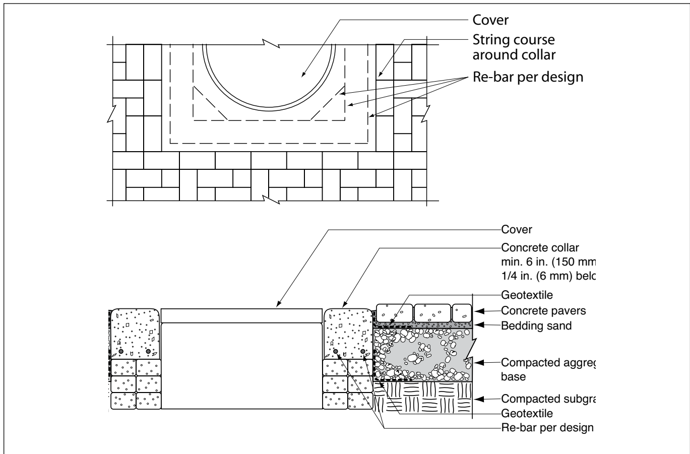
Figure 9. Utility cover.
